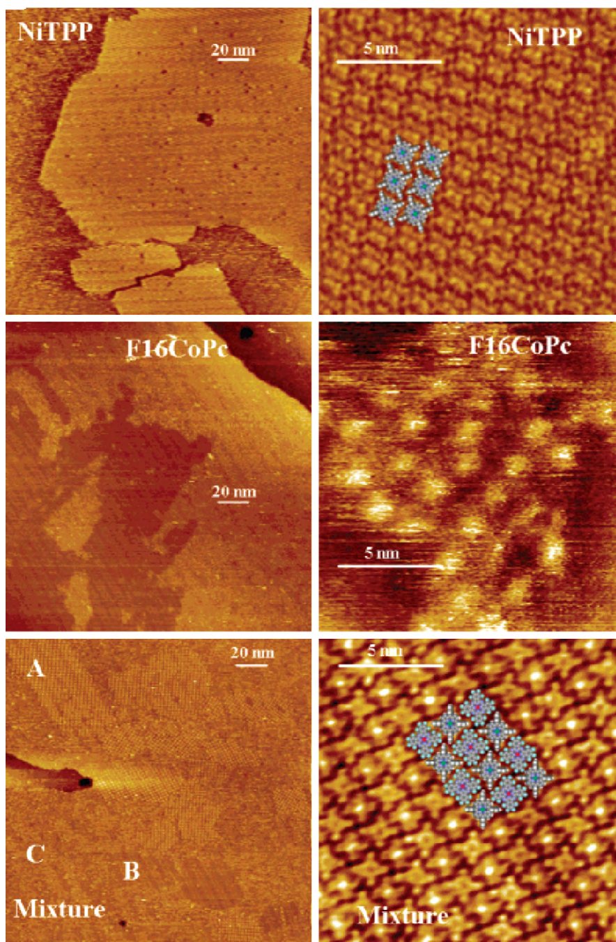
Fig. 4. Large planar macrocycles such as porphyrins and phthalocyanines tend to adsorb cofacially on surfaces such as highly ordered pyrolytic graphite (HOPG), Au(III), NaCl, and other atomically smooth substrates. Here Ni(TPP) and PcF 16 are deposited on HOPG as well as a 2:1 mixture. Reproduced from Ref. [115] with permission of the copyright holders.
